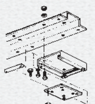
801951 RK-S Mounting Bracket
