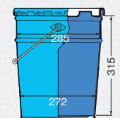
Open Head Tapered Pail
