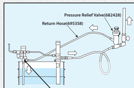
802781 RL-SA Return Hose Adapter
