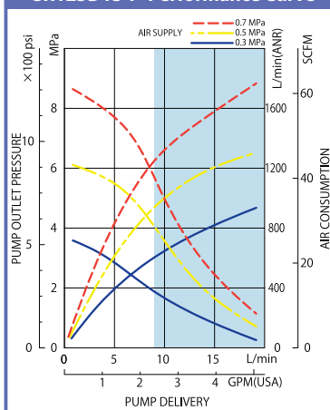
SR125D13-P Performance Curve
