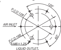
Mounting Dimensions
